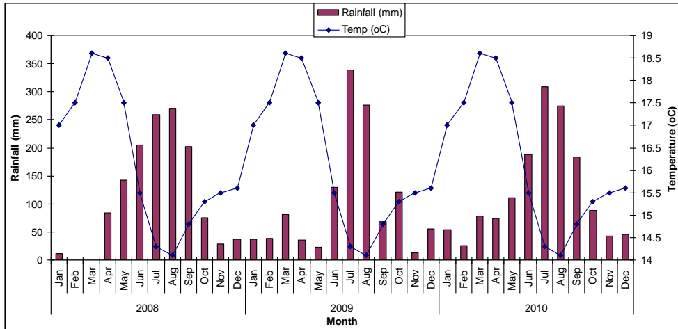
Figure 5: Climate of the study area during the study period, including the previous year (2008)
