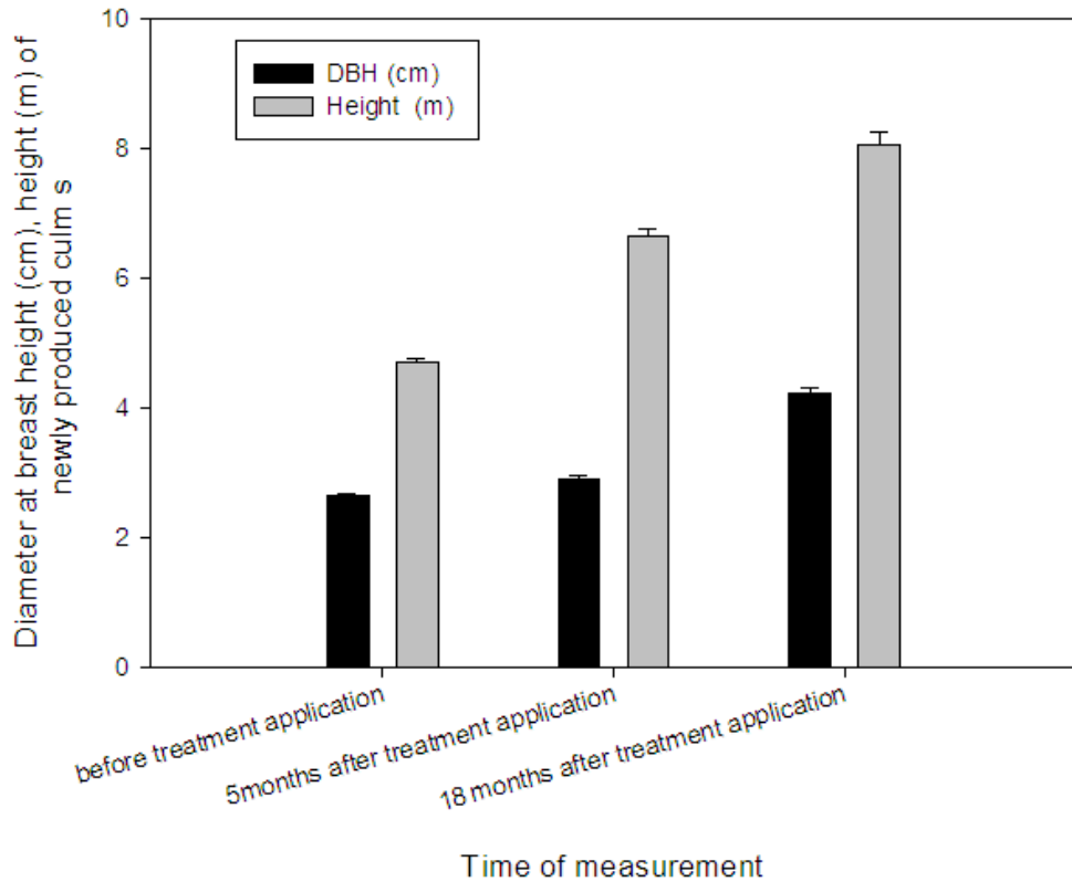
Figure 4: Diameter and height growth of newly recruited shoots across years
