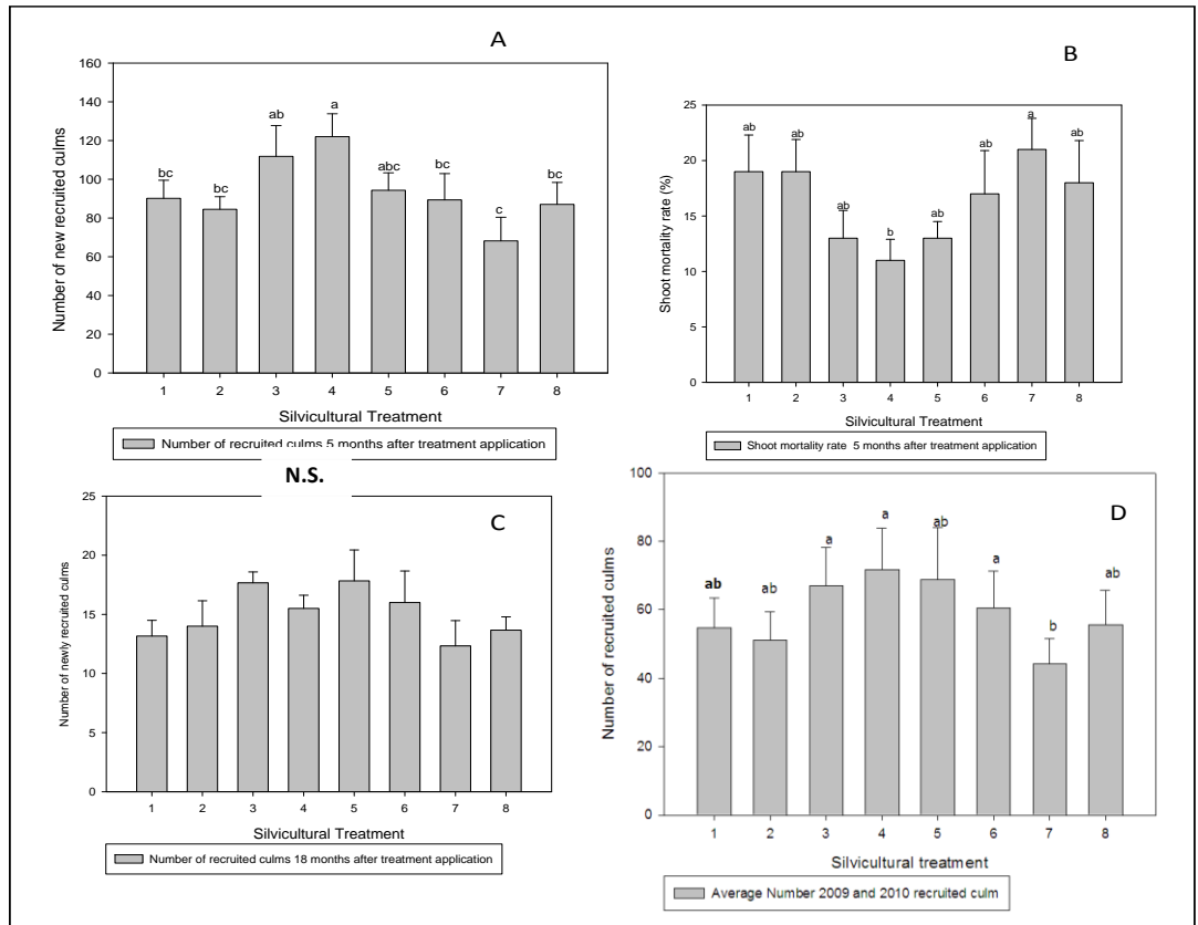
Figure 2. Culm recruitment and shoot mortality as affected by application of silvicultural management techniques (treatments): (A) culm recruitment 5 months after treatment; (B) shoot mortality rate 5 months after treatment; (C) culm recruitment 18 months after treatment; (D) two years average culm recruitment (5 and 18 months after treatment)
